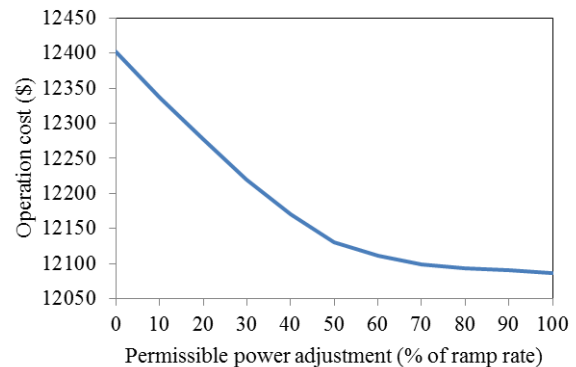
Fig. 5 Microgrid operation cost as a function of permissible power adjustment
