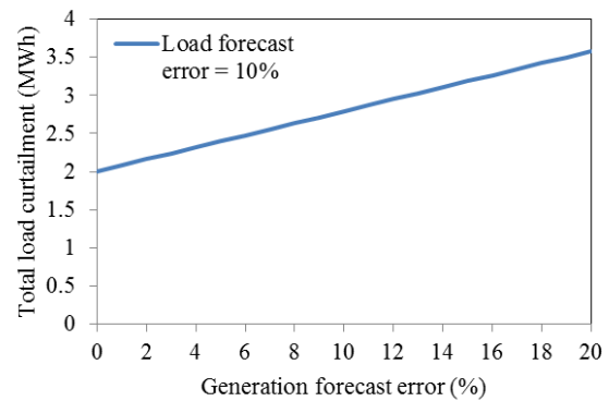
Fig. 4 Total load curtailment as a function of generation forecast error
